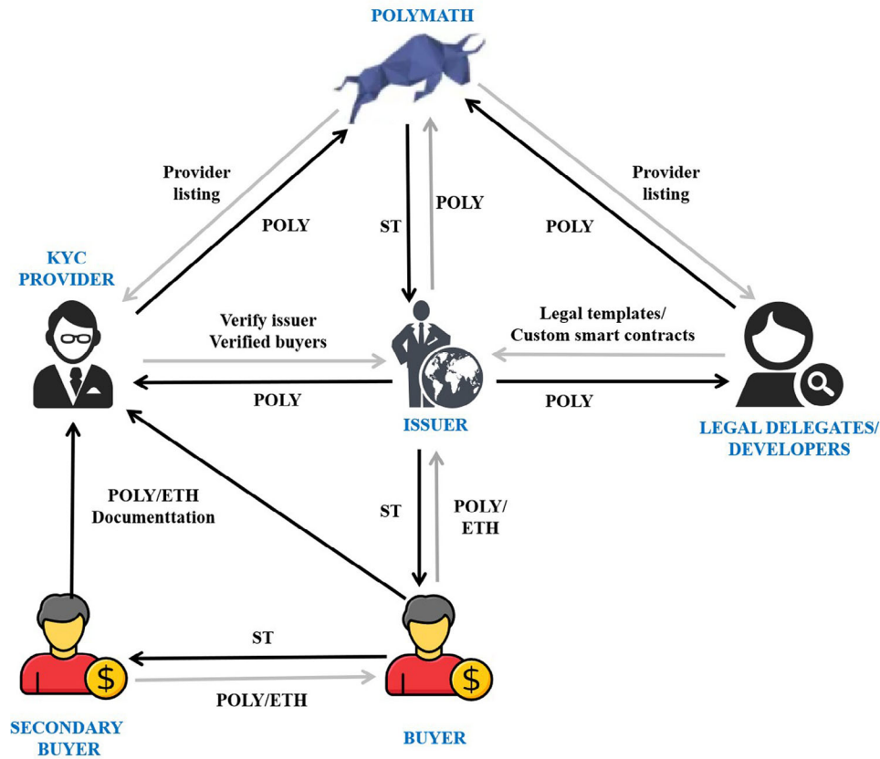
FIGURE 3 The security token issuance and transaction process on the Polymath platform.
